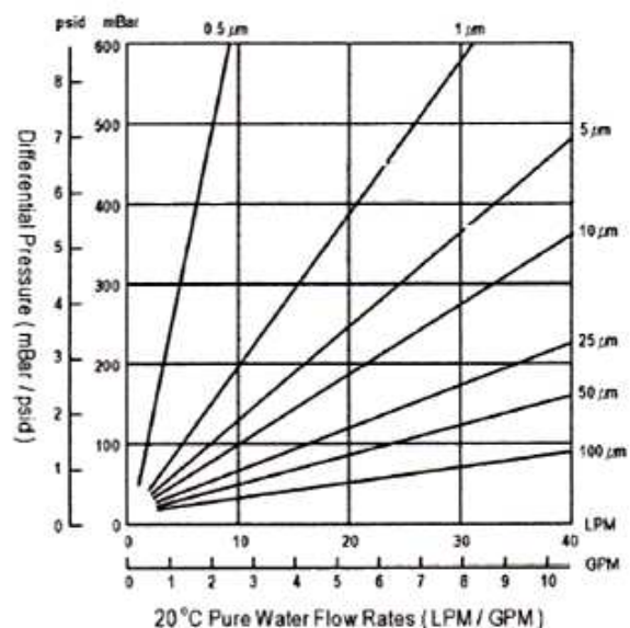
Typical Water Flow Rates (10 inch Length)
